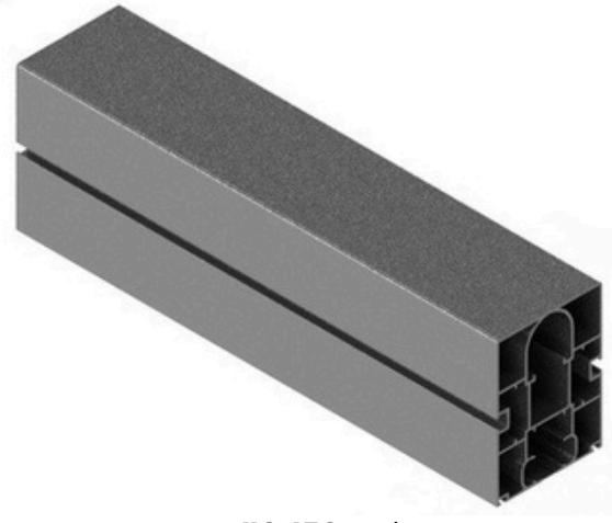
110x150 Lima Ray 110x150 Rail
